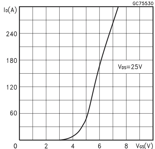
Figure 6. Transfer Characteristics
